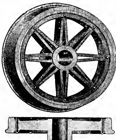
Figs. 5294-5295. DOUBLE-SPOKE WHEEL. Mansel Retaining-rings.
